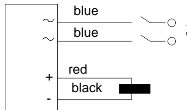
Connection of the standard rectifiers
